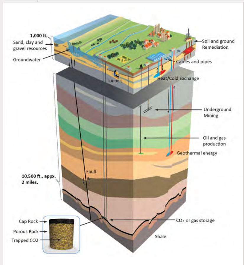
Conceptual 3D geologic diagram showing CO 2 injection and storage co-located among other uses and interests. Geologic carbon sequestration works by injecting CO 2 deep below the earth's surface into a naturally-occurring formation of porous rock. Source: Modified from TNO, Geological Survey of the Netherlands, and the Global CCS Institute, California Department of Conservation. https://www.conservation.ca.gov/cgs/gcs . 2023.
